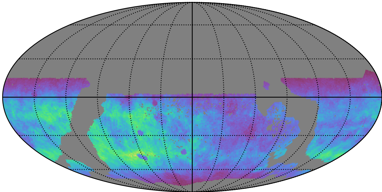
too_elab_r16_d2_gz_v3.4_10yrs WFD g band: Normalized Teff
