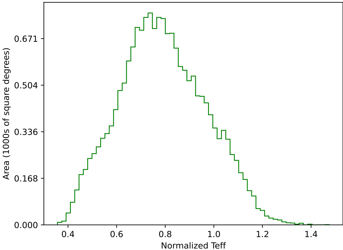
too_elab_r16_d2_gz_v3.4_10yrs WFD g band: Normalized Teff
