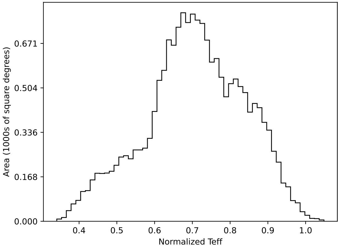
too_elab_r16_d2_gz_v3.4_10yrs WFD all bands: Normalized Teff
