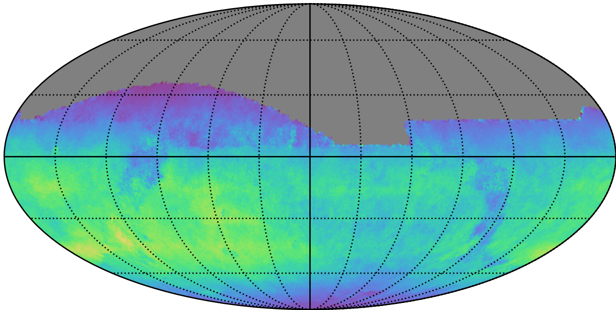
too_elab_r16_d2_gz_v3.4_10yrs All sky z band: Normalized Teff
