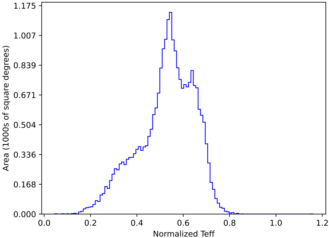
too_elab_r16_d2_gz_v3.4_10yrs All sky y band: Normalized Teff
