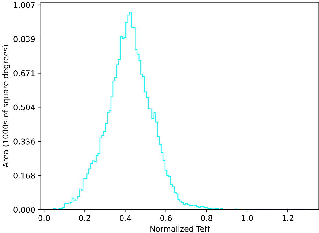
too_elab_r16_d2_gz_v3.4_10yrs All sky u band: Normalized Teff
