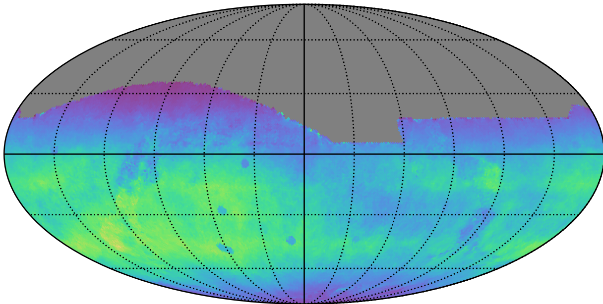
too_elab_r16_d2_gz_v3.4_10yrs All sky r band: Normalized Teff
