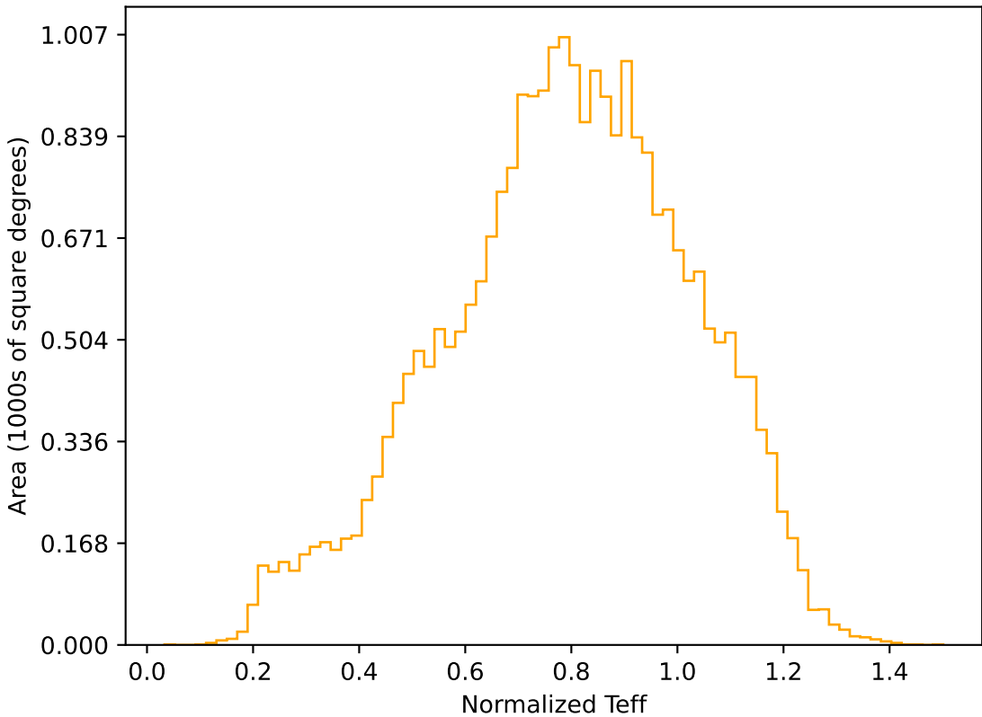
too_elab_r16_d2_gz_v3.4_10yrs All sky r band: Normalized Teff
