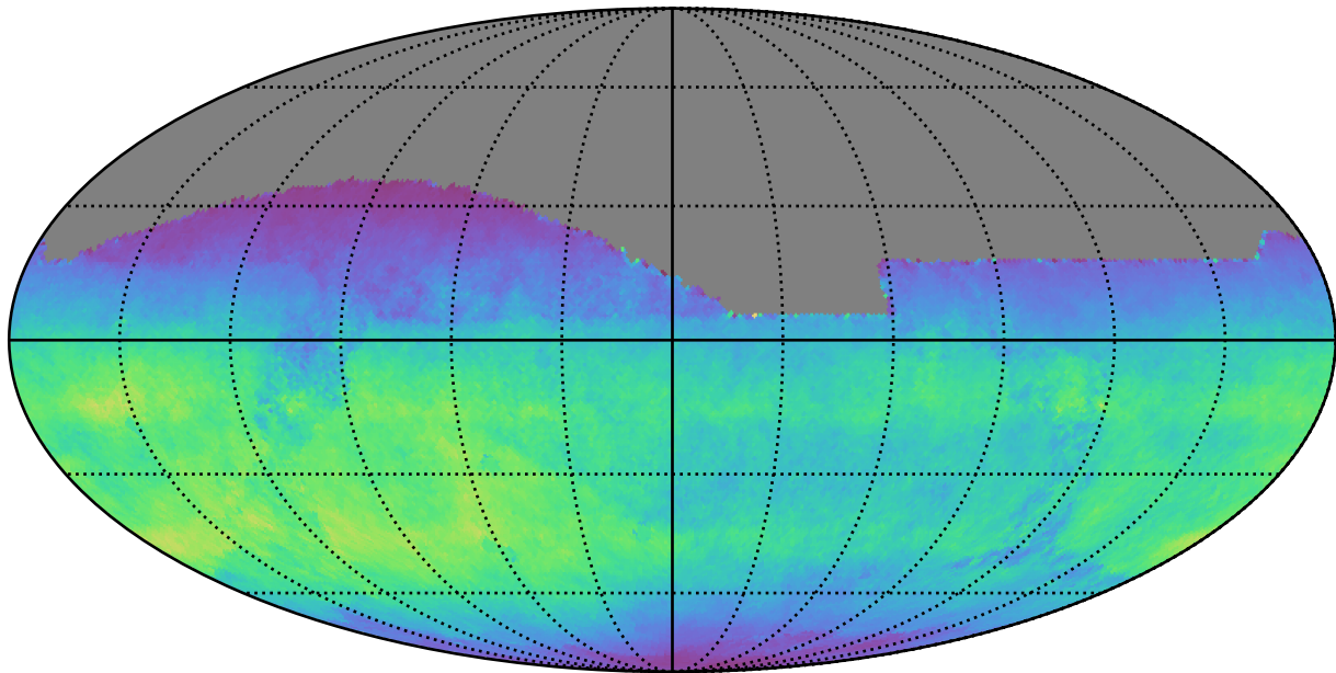
too_elab_r16_d2_gz_v3.4_10yrs All sky i band: Normalized Teff
