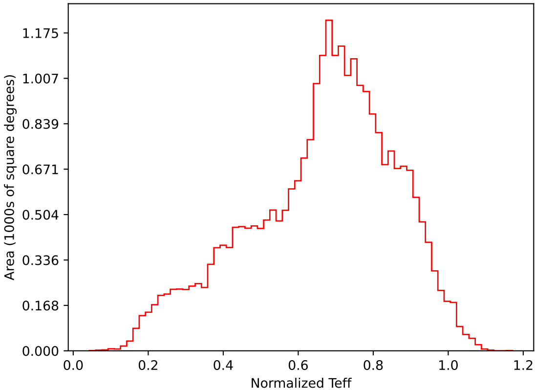
too_elab_r16_d2_gz_v3.4_10yrs All sky i band: Normalized Teff
