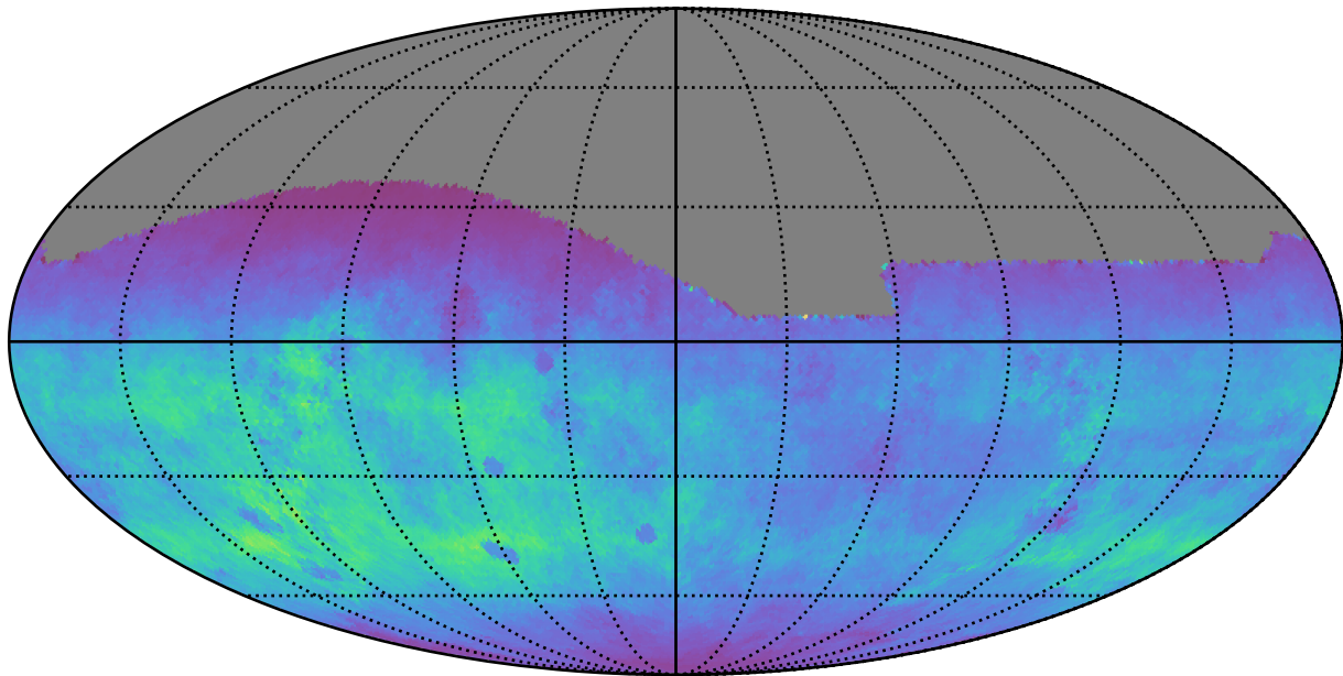
too_elab_r16_d2_gz_v3.4_10yrs All sky g band: Normalized Teff
