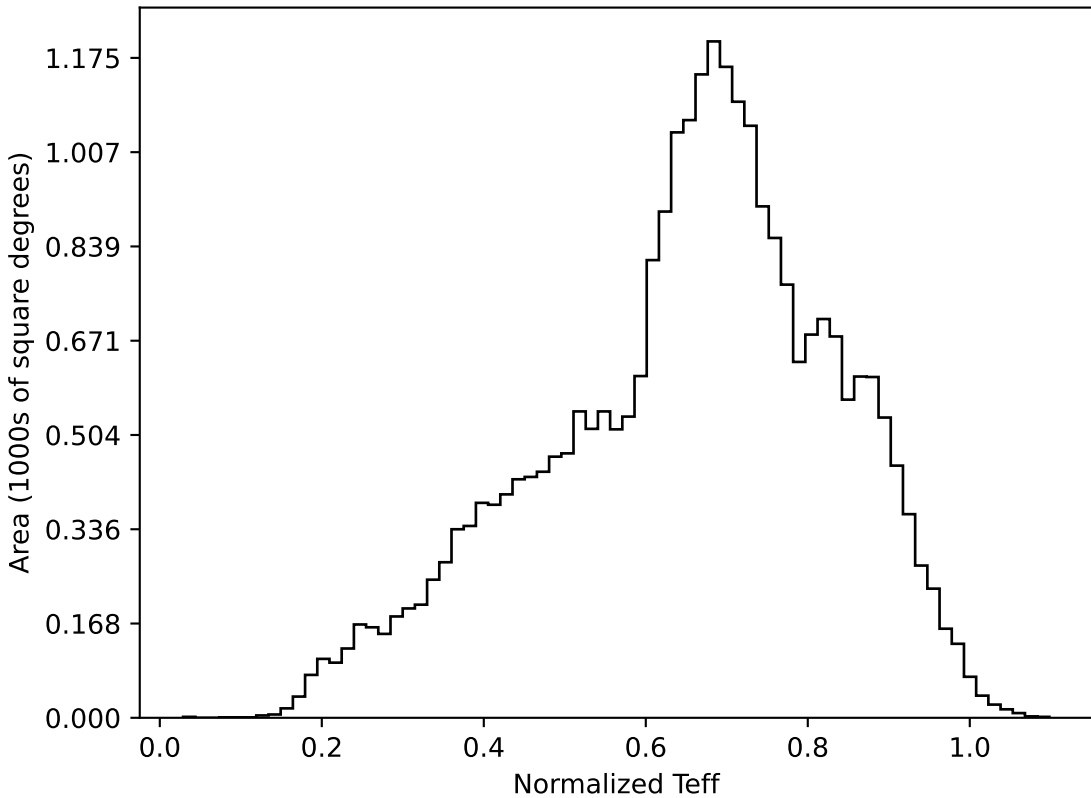
too_elab_r16_d2_gz_v3.4_10yrs All sky all bands: Normalized Teff
