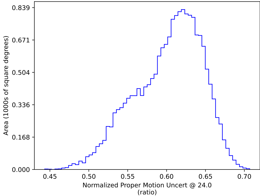
too_elab_r16_d2_gz_v3.4_10yrs WFD: Normalized Proper Motion Uncert @ 24.0
