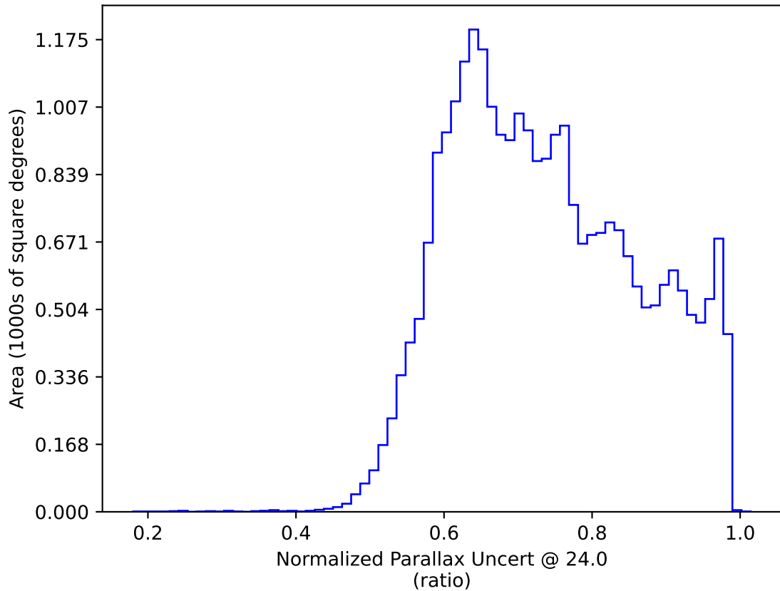
too_elab_r16_d2_gz_v3.4_10yrs All sky: Normalized Parallax Uncert @ 24.0
