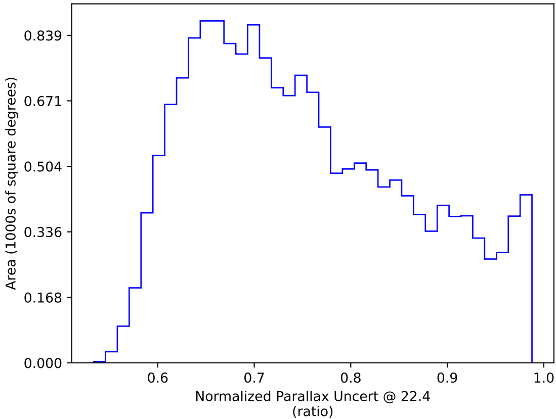
too_elab_r16_d2_gz_v3.4_10yrs WFD: Normalized Parallax Uncert @ 22.4
