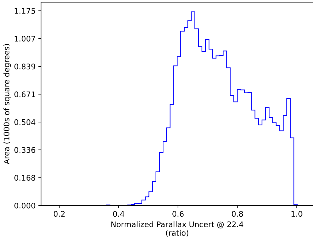
too_elab_r16_d2_gz_v3.4_10yrs All sky: Normalized Parallax Uncert @ 22.4
