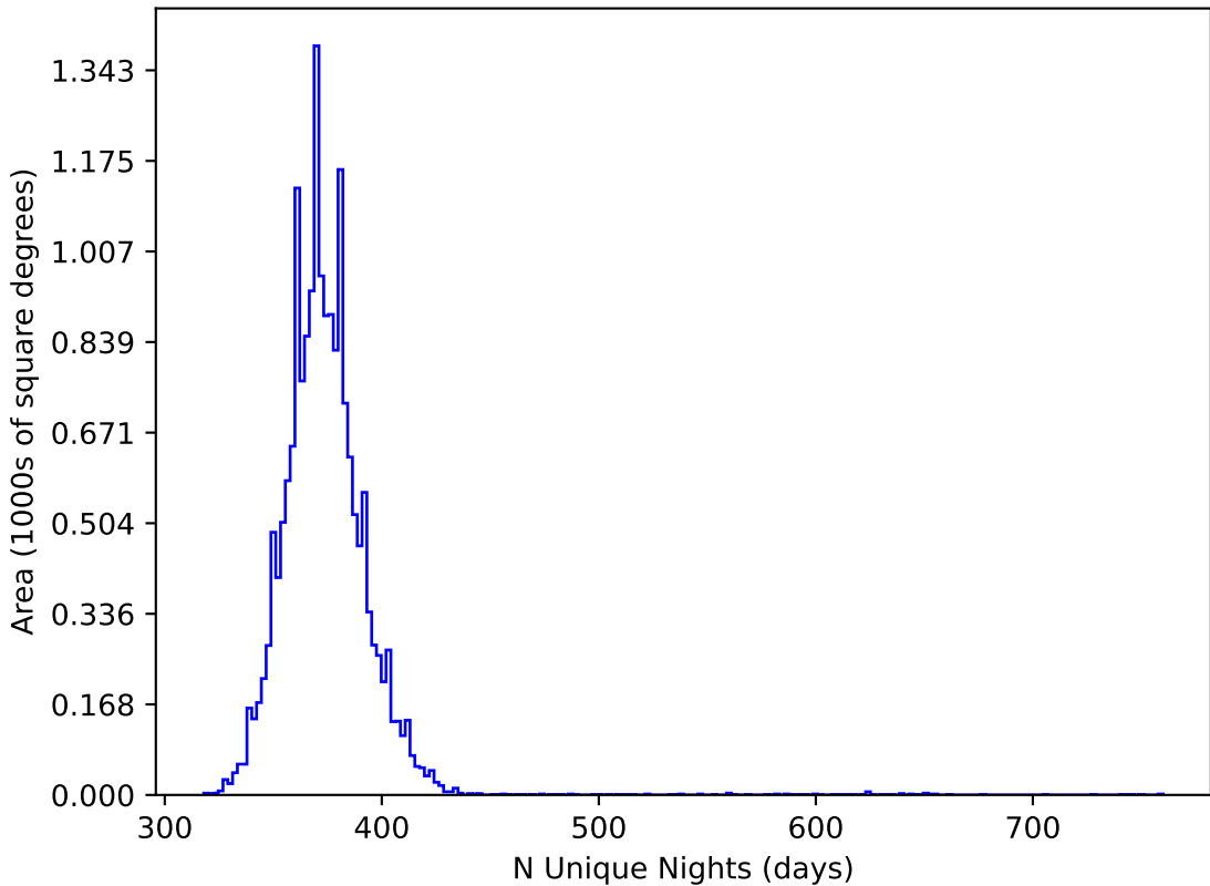
too_elab_r16_d2_gz_v3.4_10yrs WFD all bands: N Unique Nights
