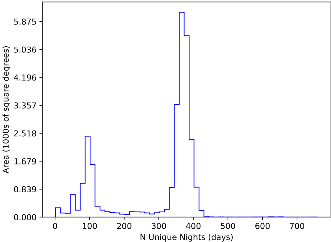
too_elab_r16_d2_gz_v3.4_10yrs All sky all bands: N Unique Nights
