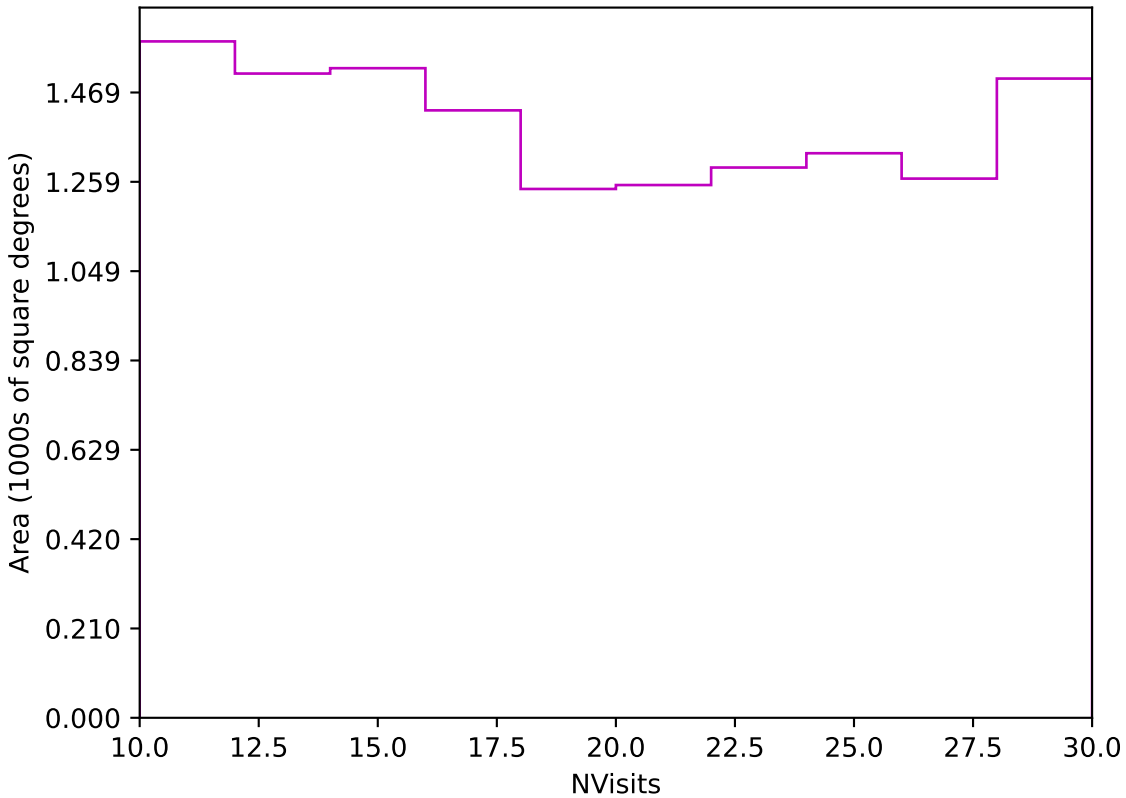
too_elab_r16_d2_gz_v3.4_10yrs Yr 3-4 z band: NVisits
