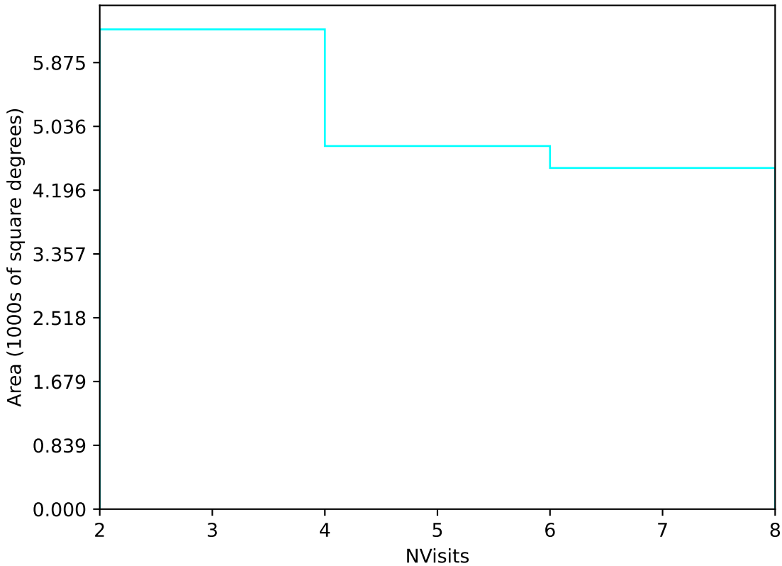
too_elab_r16_d2_gz_v3.4_10yrs Yr 3-4 u band: NVisits
