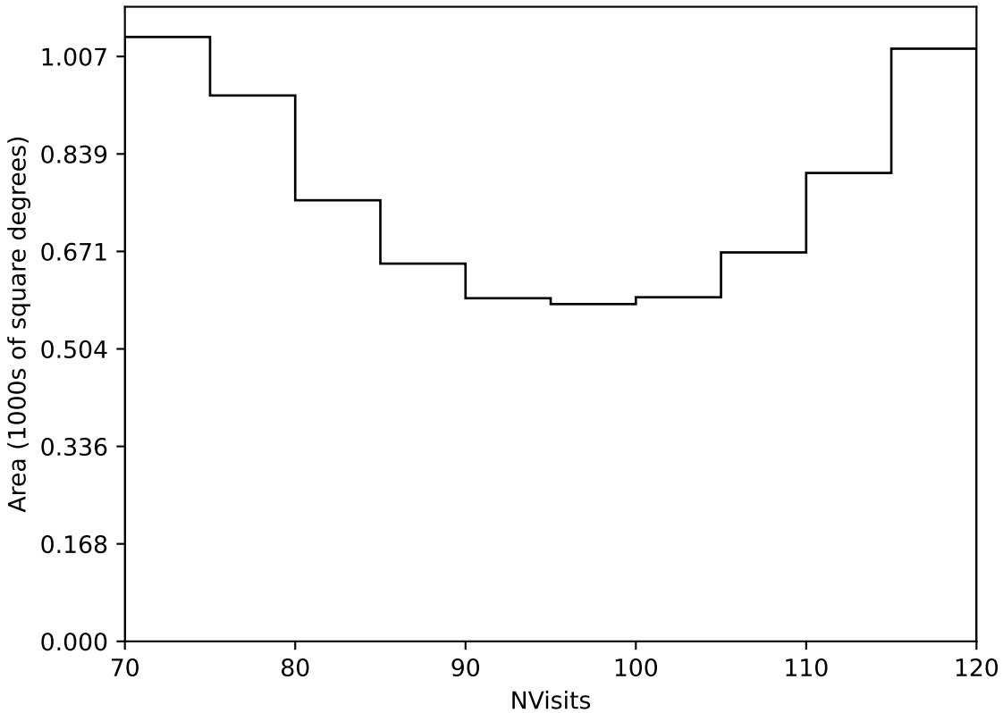
too_elab_r16_d2_gz_v3.4_10yrs Yr 3-4 all bands: NVisits
