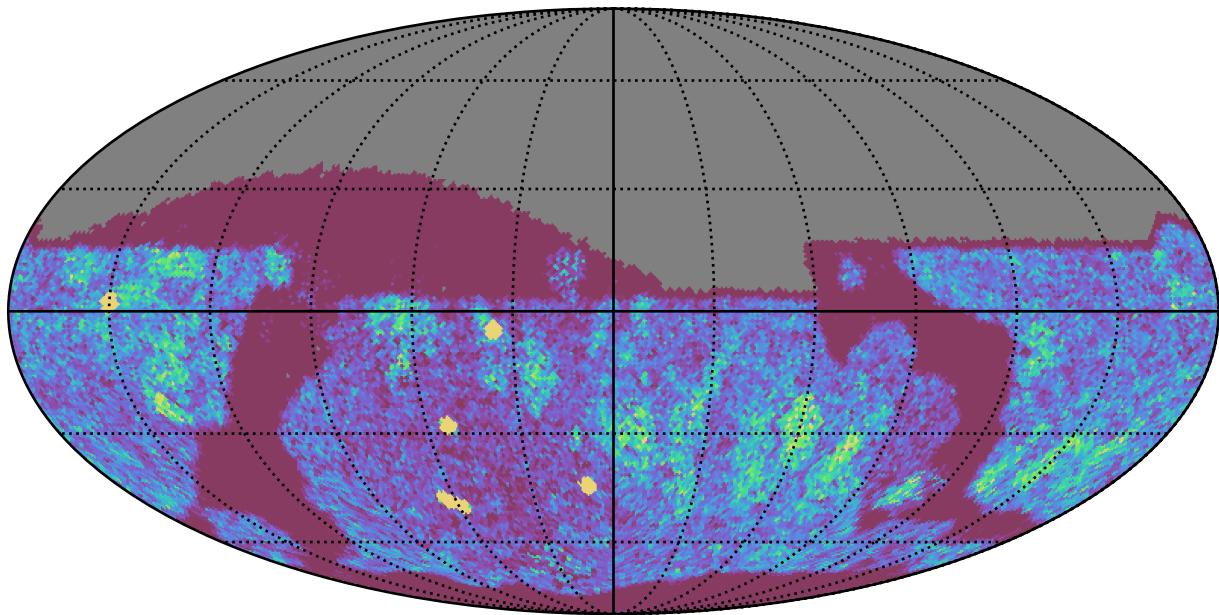
too_elab_r16_d2_gz_v3.4_10yrs Yr 1 z band: NVisits
