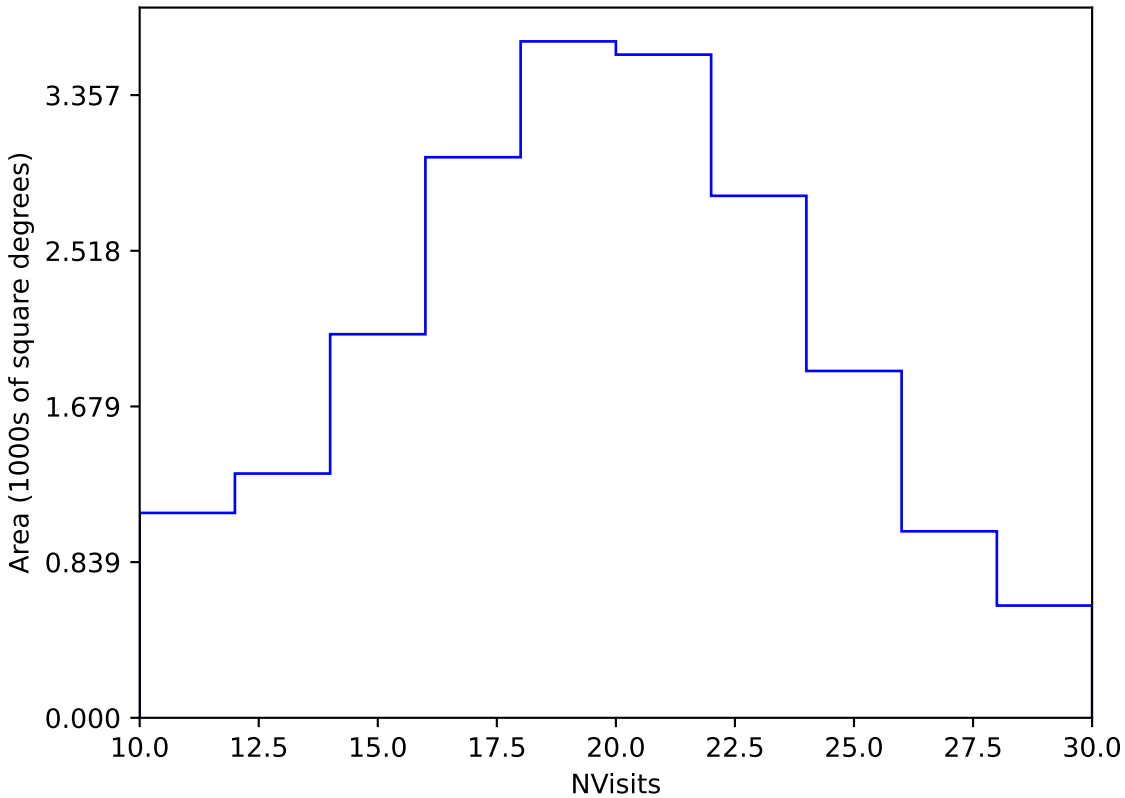
too_elab_r16_d2_gz_v3.4_10yrs Yr 1 y band: NVisits
