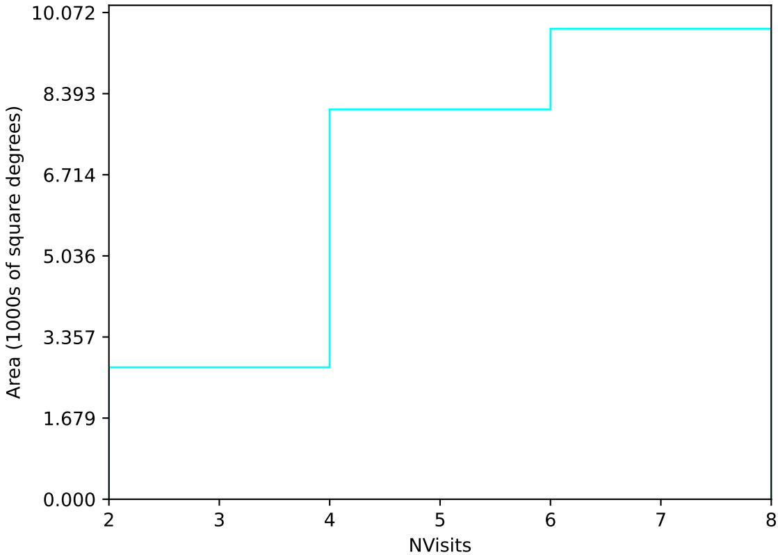
too_elab_r16_d2_gz_v3.4_10yrs Yr 1 u band: NVisits
