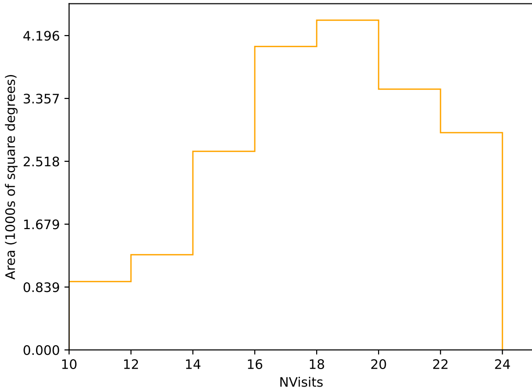
too_elab_r16_d2_gz_v3.4_10yrs Yr 1 r band: NVisits
