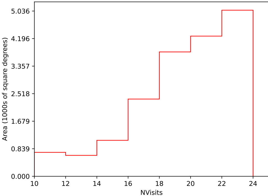
too_elab_r16_d2_gz_v3.4_10yrs Yr 1 i band: NVisits
