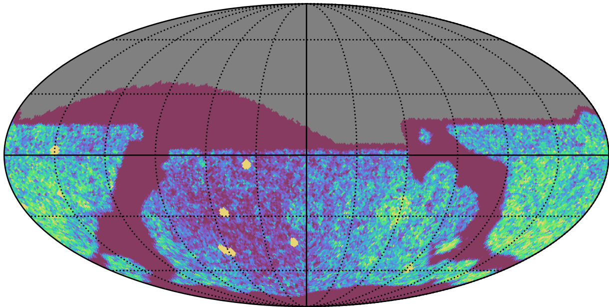
too_elab_r16_d2_gz_v3.4_10yrs Yr 1 all bands: NVisits
