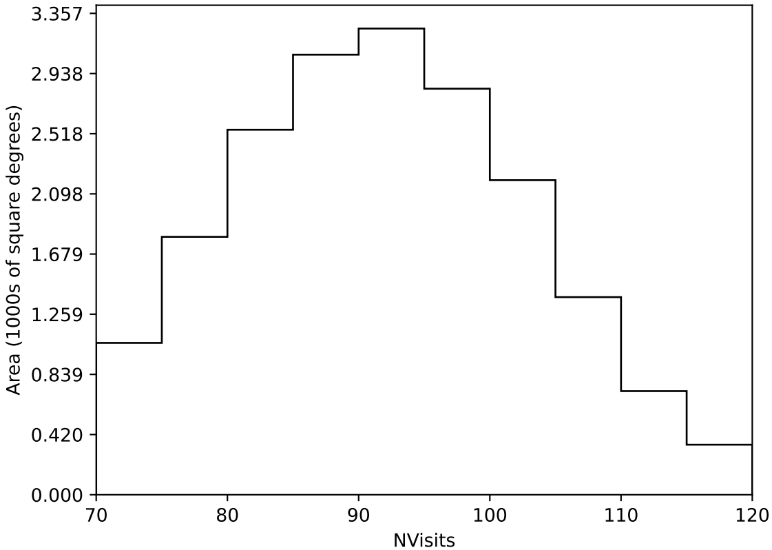
too_elab_r16_d2_gz_v3.4_10yrs Yr 1 all bands: NVisits
