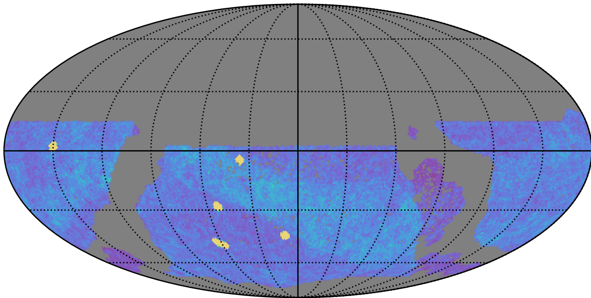
too_elab_r16_d2_gz_v3.4_10yrs WFD z band: NVisits
