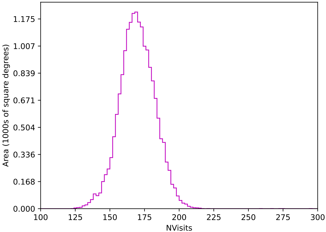
too_elab_r16_d2_gz_v3.4_10yrs WFD z band: NVisits
