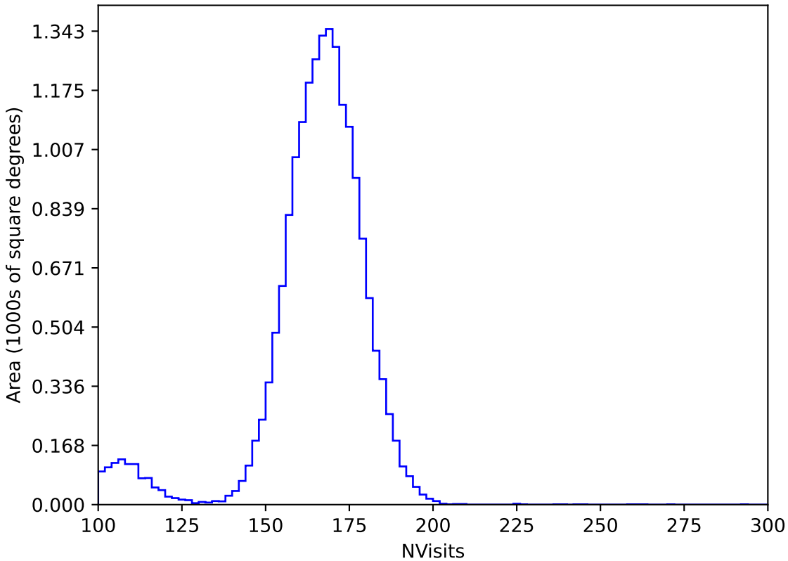
too_elab_r16_d2_gz_v3.4_10yrs WFD y band: NVisits
