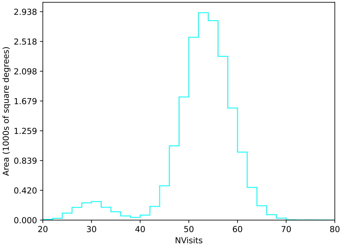
too_elab_r16_d2_gz_v3.4_10yrs WFD u band: NVisits
