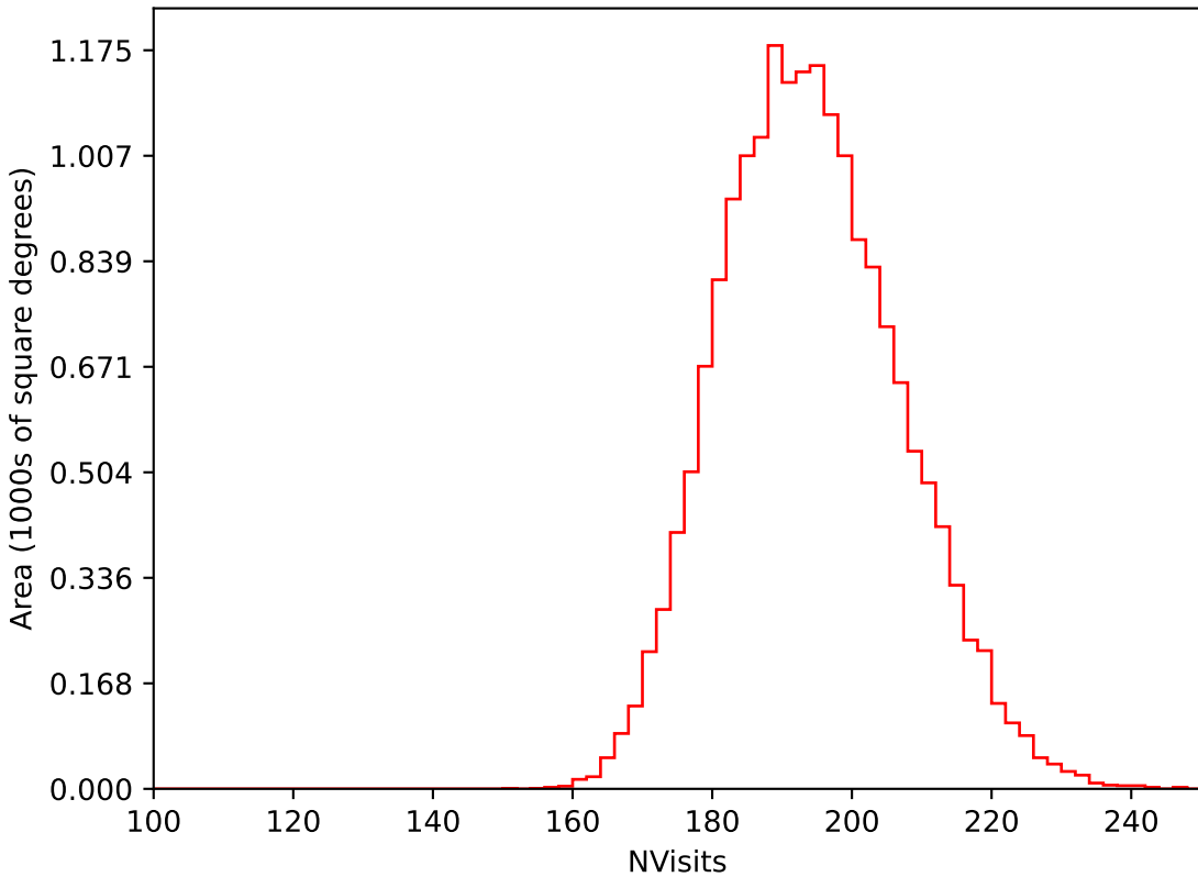
too_elab_r16_d2_gz_v3.4_10yrs WFD i band: NVisits
