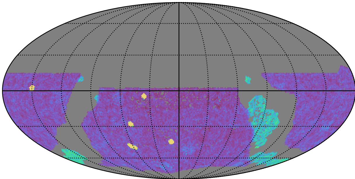
too_elab_r16_d2_gz_v3.4_10yrs WFD g band: NVisits
