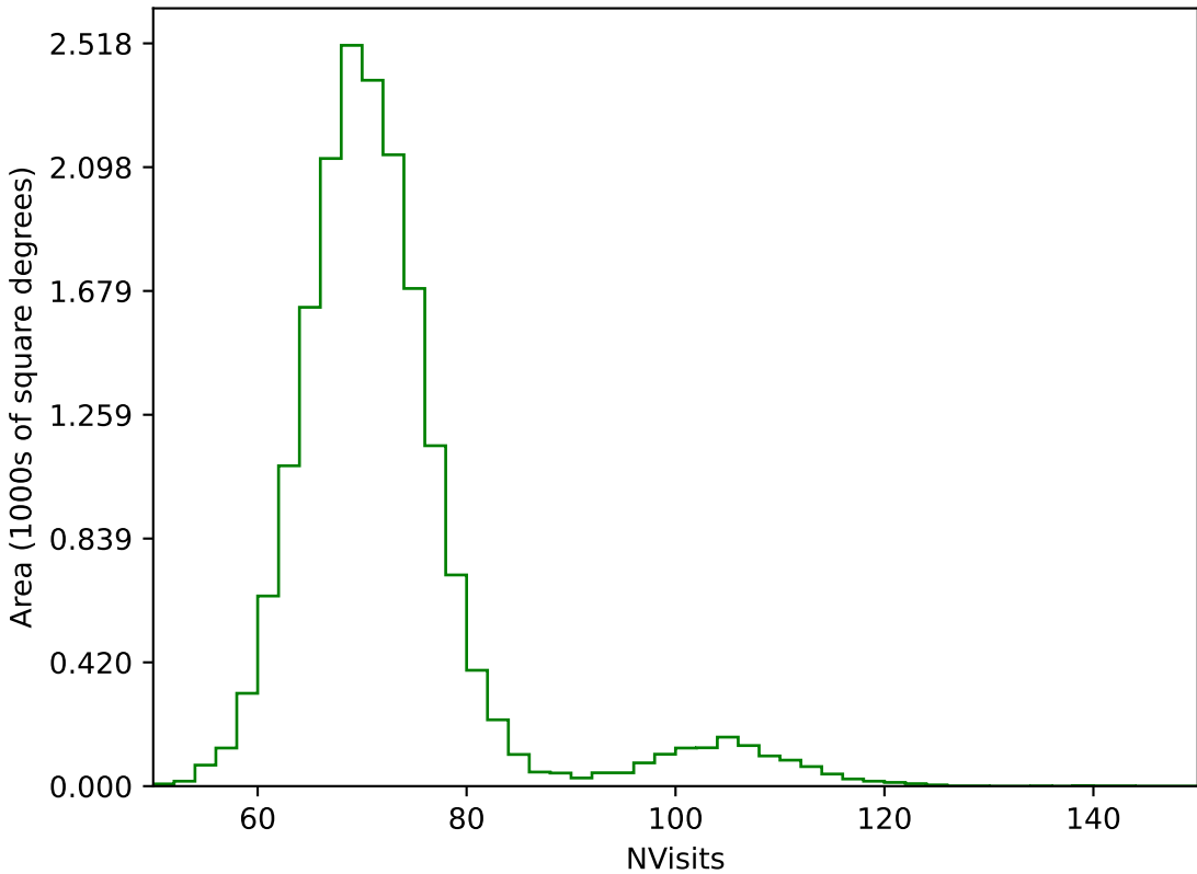
too_elab_r16_d2_gz_v3.4_10yrs WFD g band: NVisits
