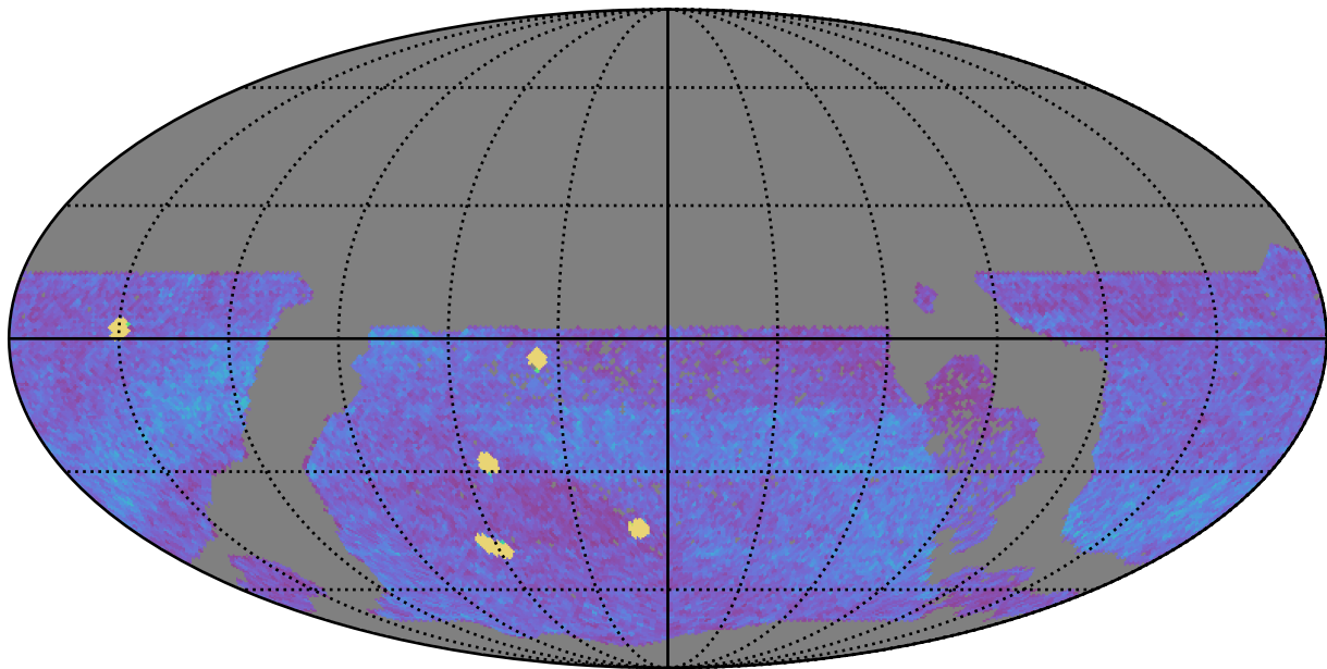
too_elab_r16_d2_gz_v3.4_10yrs WFD all bands: NVisits
