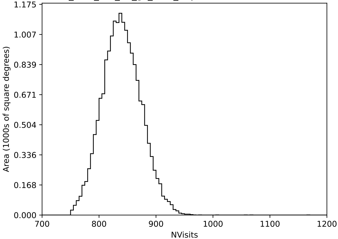
too_elab_r16_d2_gz_v3.4_10yrs WFD all bands: NVisits
