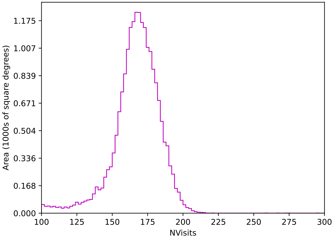
too_elab_r16_d2_gz_v3.4_10yrs All sky z band: NVisits
