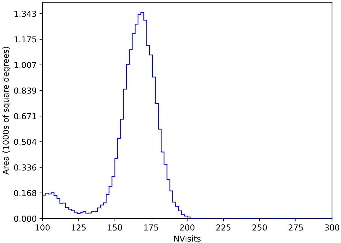
too_elab_r16_d2_gz_v3.4_10yrs All sky y band: NVisits
