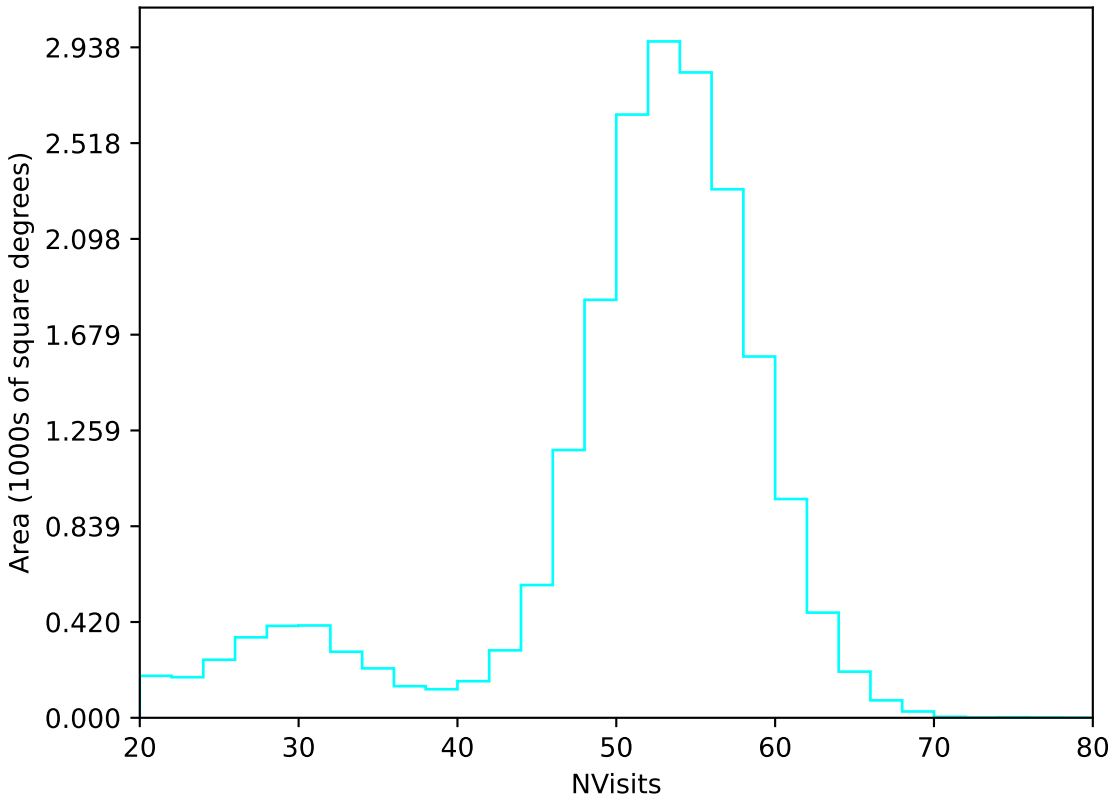
too_elab_r16_d2_gz_v3.4_10yrs All sky u band: NVisits
