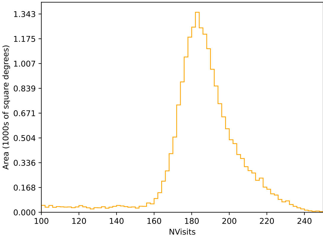
too_elab_r16_d2_gz_v3.4_10yrs All sky r band: NVisits
