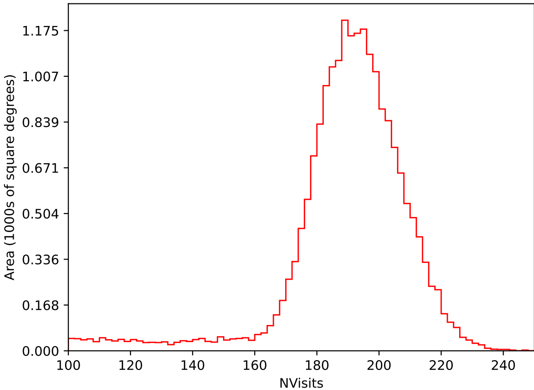
too_elab_r16_d2_gz_v3.4_10yrs All sky i band: NVisits
