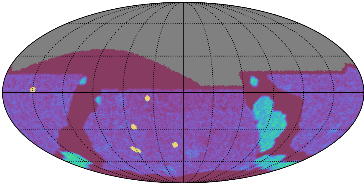
too_elab_r16_d2_gz_v3.4_10yrs All sky g band: NVisits
