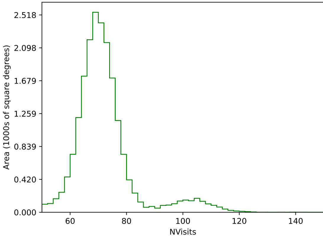
too_elab_r16_d2_gz_v3.4_10yrs All sky g band: NVisits
