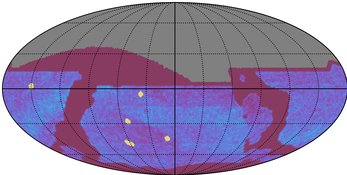
too_elab_r16_d2_gz_v3.4_10yrs All sky all bands: NVisits
