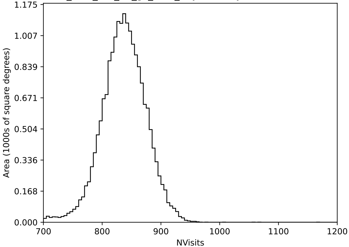
too_elab_r16_d2_gz_v3.4_10yrs All sky all bands: NVisits
