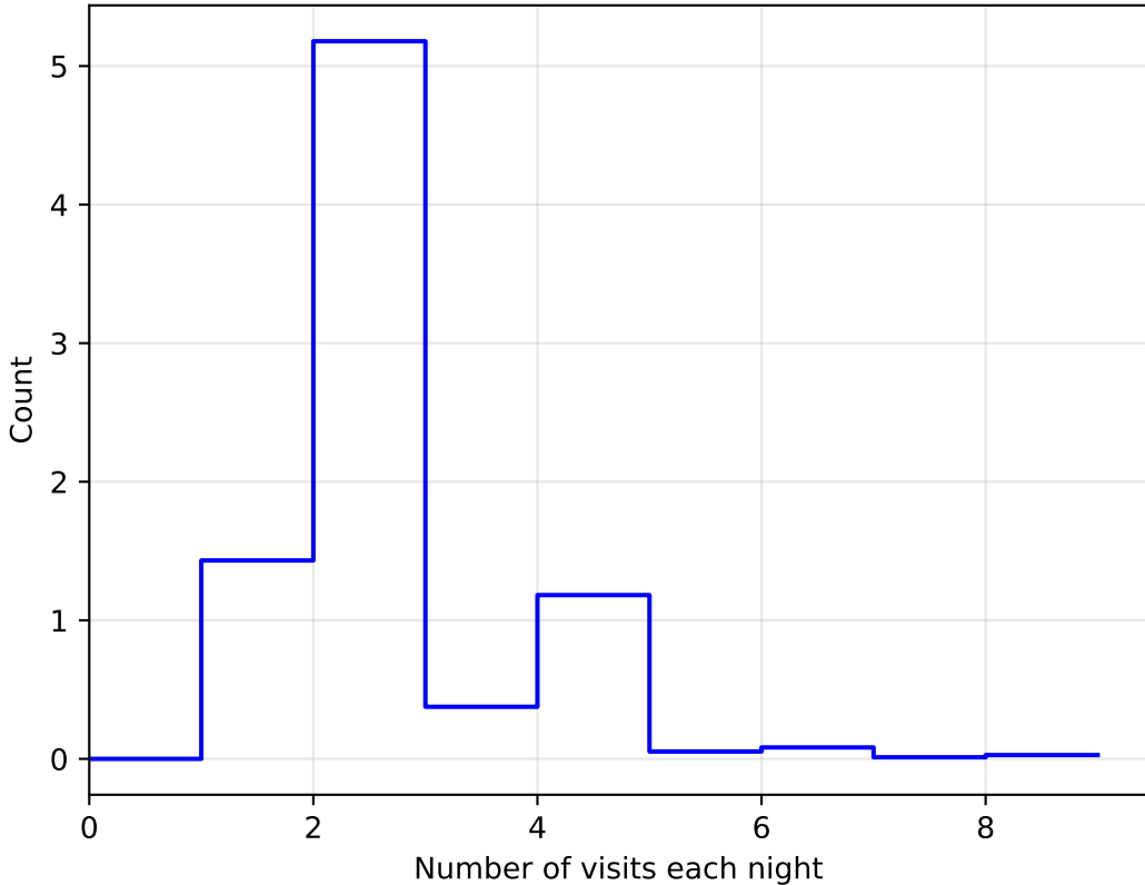
too_elab_r16_d2_gz_v3.4_10yrs WFD: NVisitsPerNight
