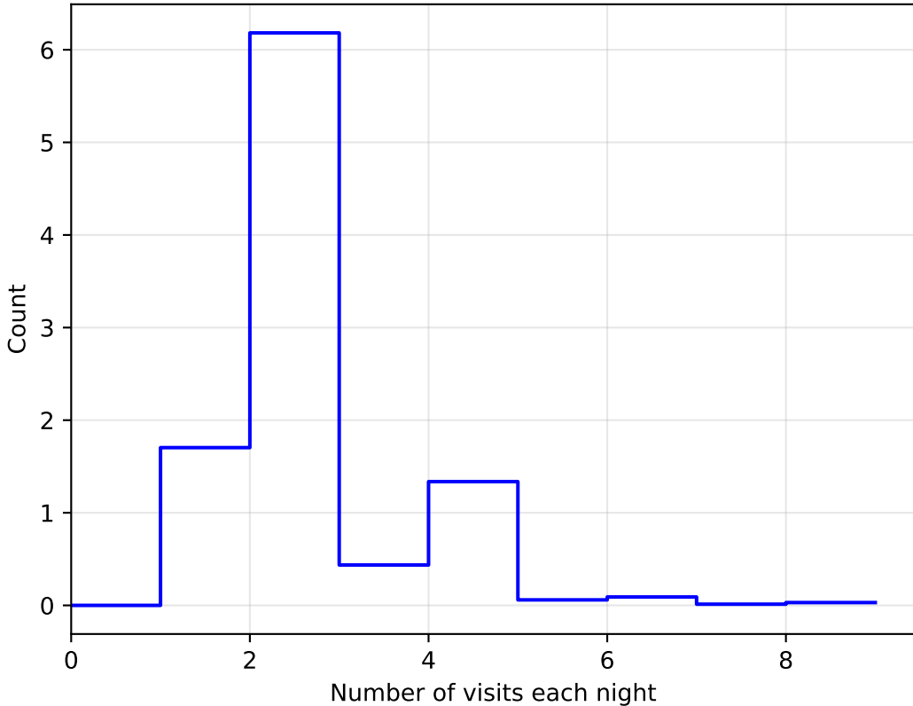
too_elab_r16_d2_gz_v3.4_10yrs All sky: NVisitsPerNight
