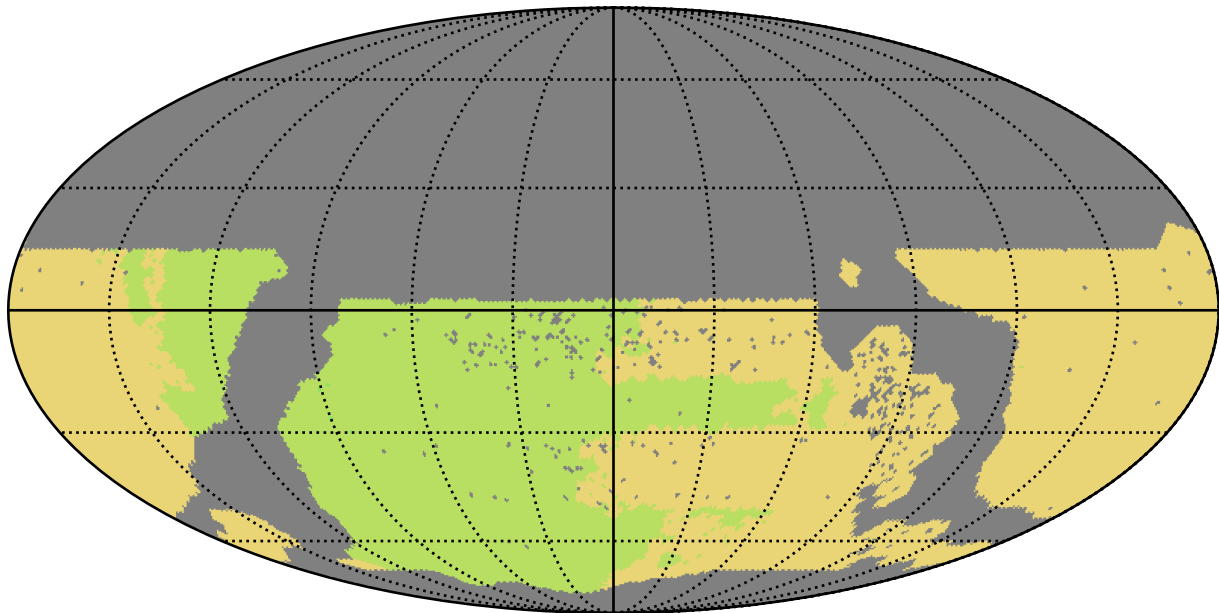
too_elab_r16_d2_gz_v3.4_10yrs WFD all bands: NSeasons
