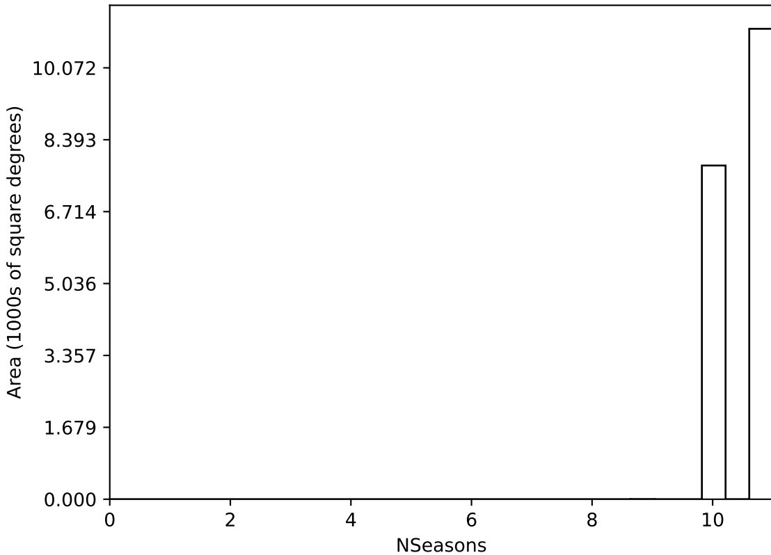
too_elab_r16_d2_gz_v3.4_10yrs WFD all bands: NSeasons
